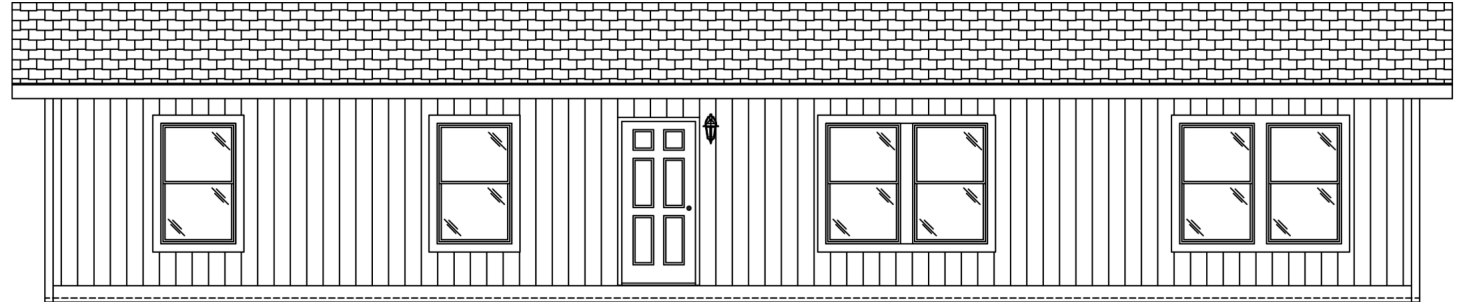
FRONT SIDEWALL
